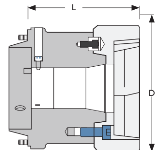
A2-5 16C ADAPTER WITH 4 ED CLOSER
