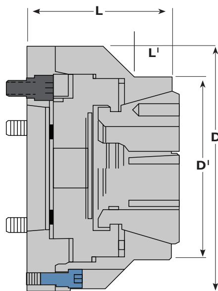
42 & 65MM SYSTEMS
