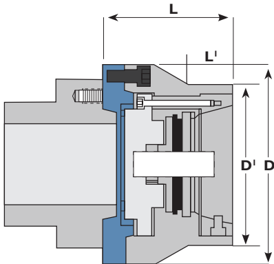
80MM SYSTEMS
